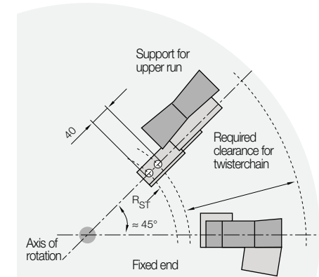
Mounting position for one support
