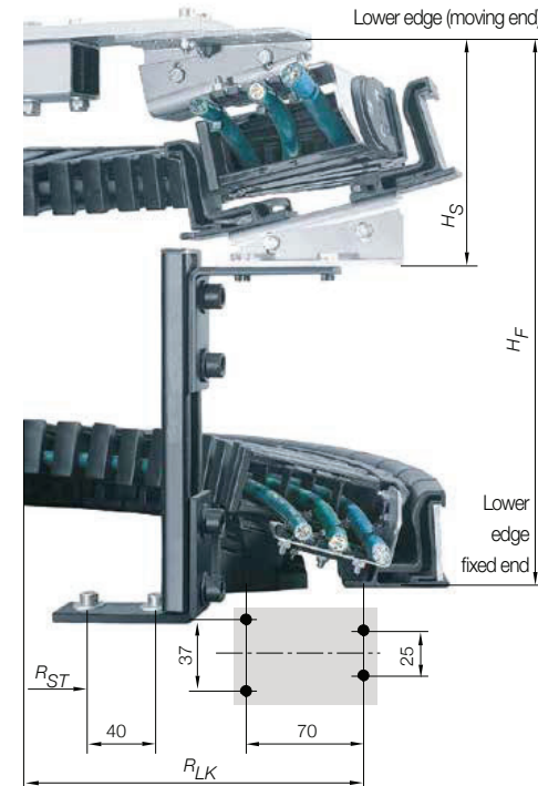
Mounting position for one support
