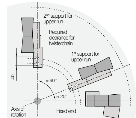
Mounting position for two supports
