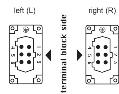
female inserts (CTF and CTSEF)
