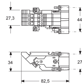
male inserts (CTM and CTSEM)
