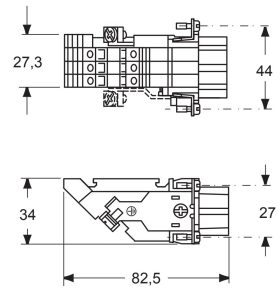
female inserts (CTF and CTSEF)
