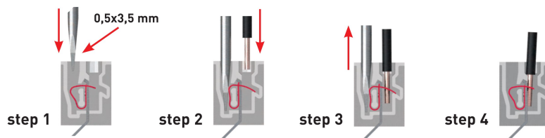
Connection technology with spring terminal
