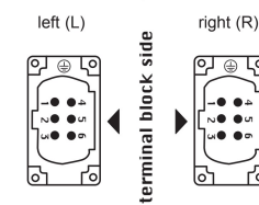
male inserts (CTM and CTSEM)
